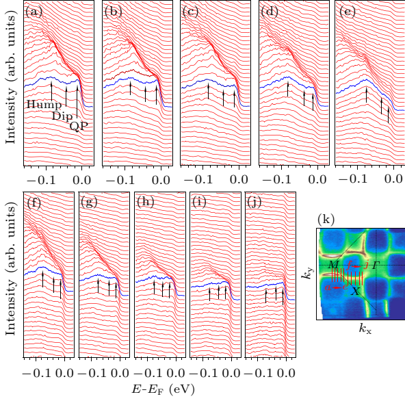
Fig. 3. Plots of EDCs along the 10 cuts marked as red lines (a)–(e) and (f)–(j) in the BZ in (k). (k) ARPES intensity plot of FSs recorded at 30 K with horizontally polarized photons.
