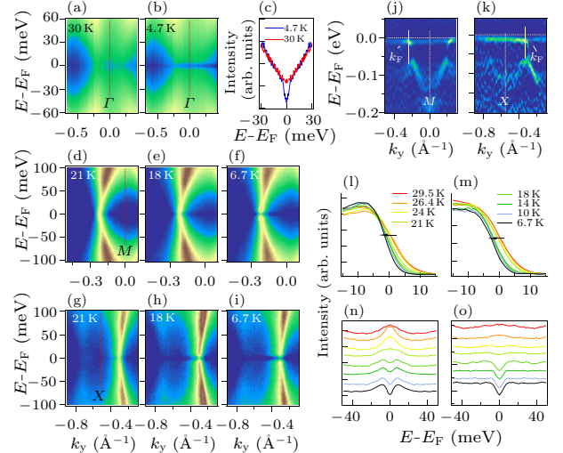
Fig. 4. [(a), (b)] Zoomed-in symmetrized intensity plots of the bands around the BZ center at 30 K and 4.7 K showing that the superconducting gap opens at low temperatures. (c) Symmetrized EDC at k_F of (a) and (b). (d)–(f) Zoomed-in symmetrized band structure around k_F of the M -centered electron-like pocket at different temperatures. (g)–(i) Zoomed-in symmetrized band structure around k_F of the X -centered hole-like pocket at different temperatures. [(j), (k)] The 2D curvature intensity plots of Ti-related bands structure around M and X . [(l), (m)] The EDCs at k_F (marked as white lines in (j) and (k), respectively) recorded at different temperatures. [(n), (o)] The symmetrized EDCs of (l) and (m) showing that the superconducting gap opens below T_c .
