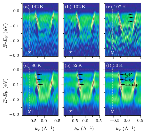
Fig. 2. The 2D curvature intensity plots of the band structure along the X – X high-symmetry line at different temperatures from 142 K to 30 K. The arrows indicate the quasiparticle peaks (QP), dips, and humps appearing at below 120 K.
