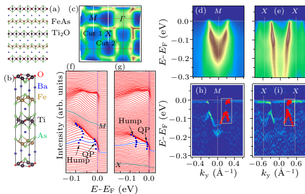
Fig. 1. (a), (b) Side view of layer structure and 3D view of the unit cell superlattice structure consisting of alternating stacking of BaFe 2 As 2 and BaTi 2 As 2 O layers. (c) Fermi surface intensity plot and indication of cut1 and cut2 in the BZ. (d) Ti-related electron-like band structure centered at M recorded along cut1. (e) Ti-related hole-like band structure centered at X recorded along cut2. (f), (g) Energy distribution curves (EDCs) of (d) and (e). The dark-blue dashed lines indicate the two branches of the Ti-related bands, and the light-blue EDCs at k_F indicate the ‘peak-dip-hump’ line shape. (h), (i) The 2D curvature intensity plots of (d) and (e), showing the renormalized polaronic state features in the white boxes.
